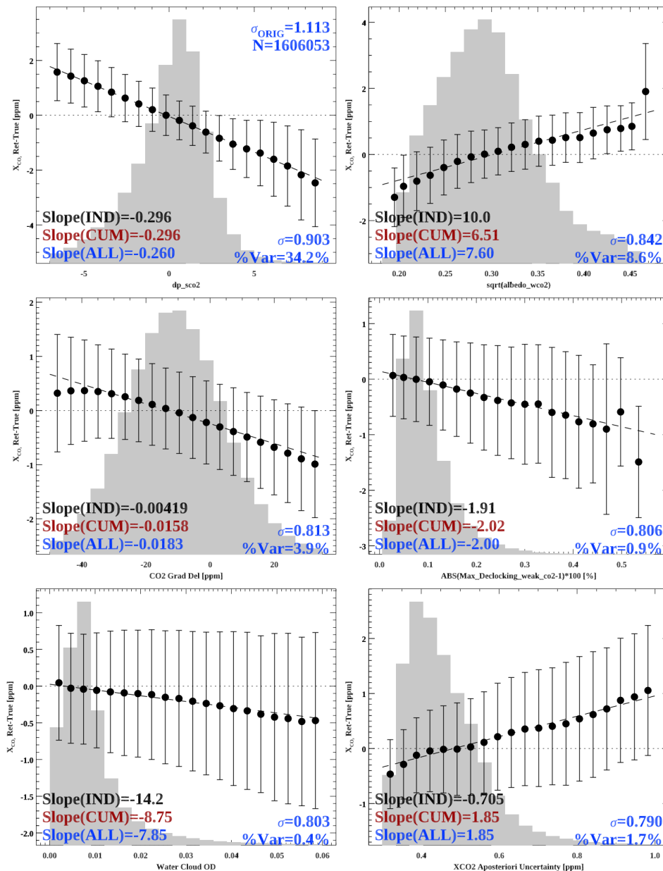
Figure 4-5: Same as Figure 4-4 but for Ocean Glint Observations.
