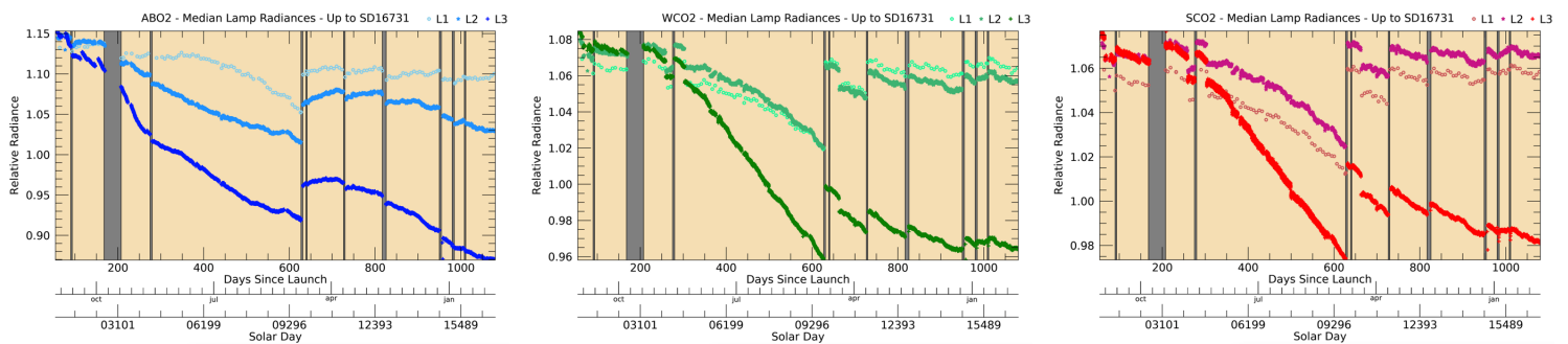
Figure 3-1: Lamp radiance trends relative to prelaunch over the course of the OCO-3 mission. The three panels are for the ABO2, WCO2, and SCO2 channels. Within each panel, different colors indicate different lamps. Lamp 3 is used roughly 12 times per day, Lamp 2 is used roughly 3 times per day, and Lamp 1 is used roughly 1 time per week.
