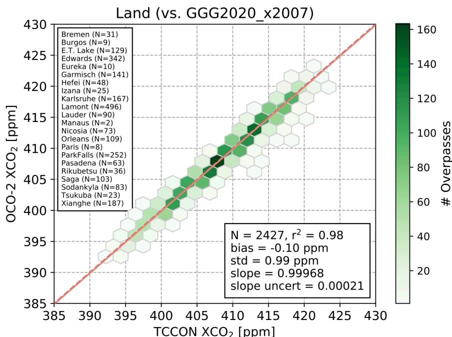
Figure 4-6: Linear Fit of OCO-2 v10 to TCCON X CO2 for a subset of land (ND+GL) mode overpasses of TCCON sites. Both Quality Filtering as well as the feature and footprint biases have been applied.
