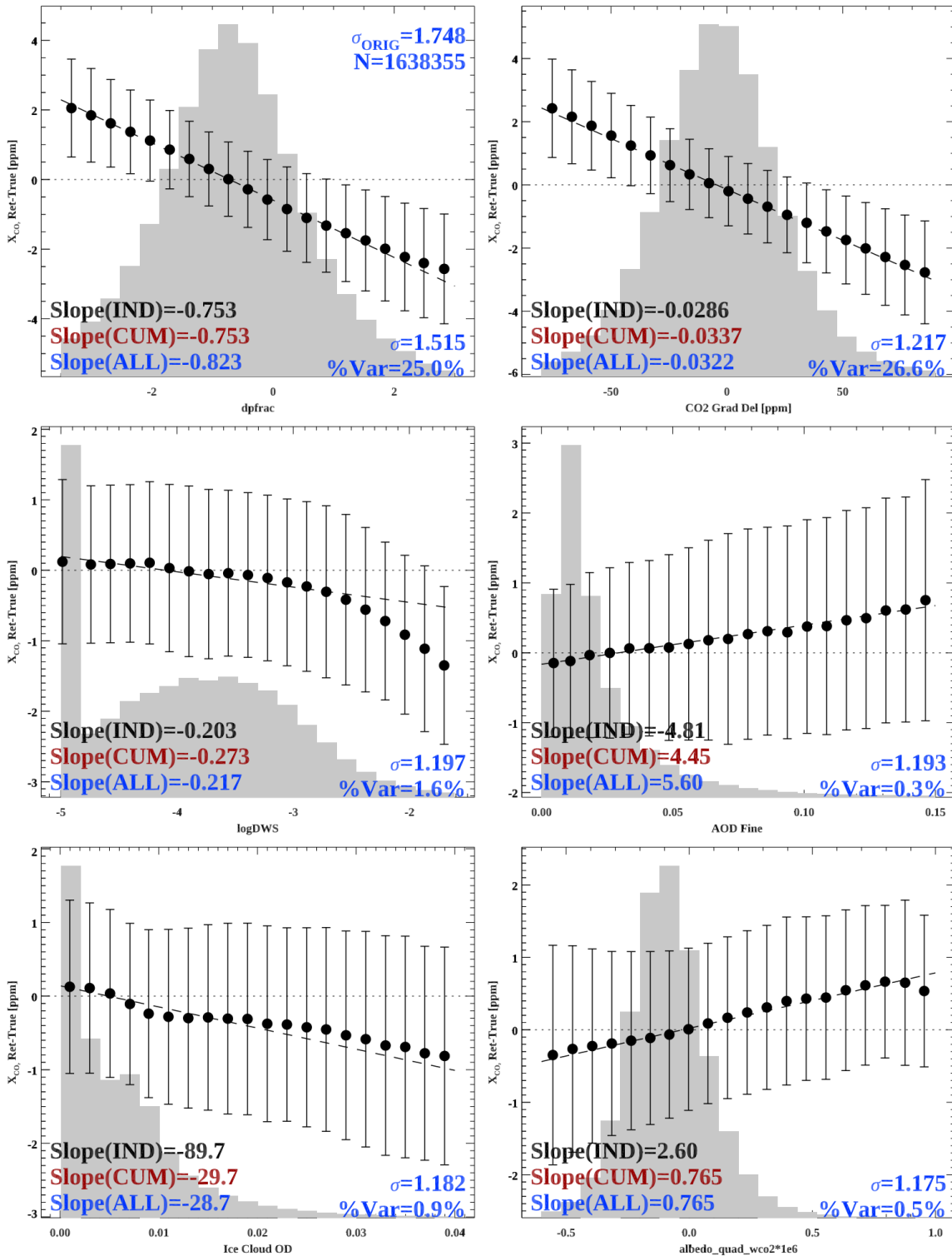
Figure 4-3: Plot of X_{CO_2} errors relative to TCCON (ggg2020) for v11.1 land nadir & glint observations. The regression coefficients for a simultaneous fit of all terms are given in blue ("ALL"), bottom left of each panel.
