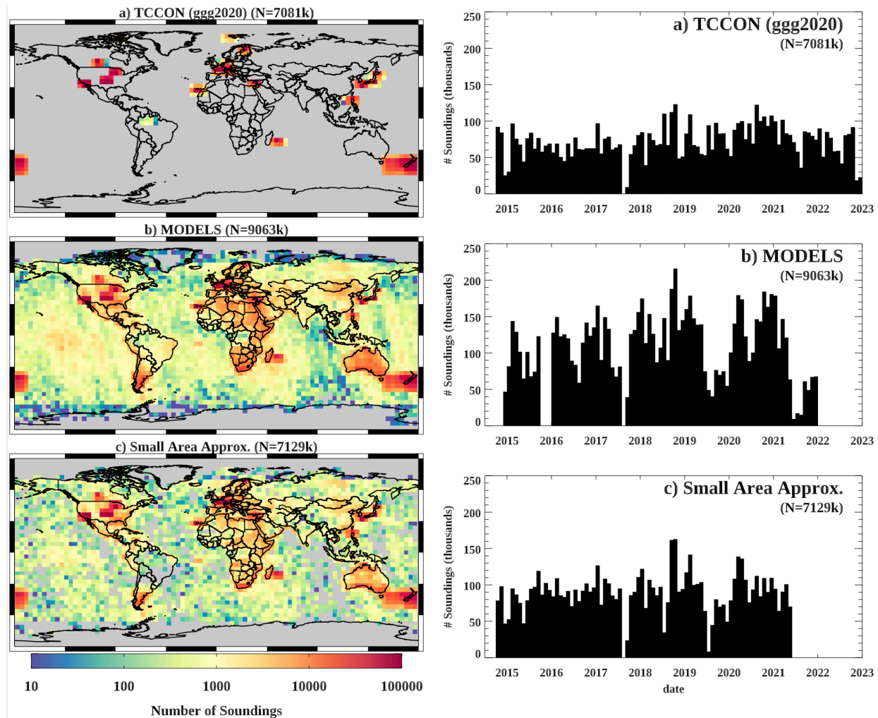
Figure 4-1: Sounding density maps and time series of soundings for the three v11 training data sets.
