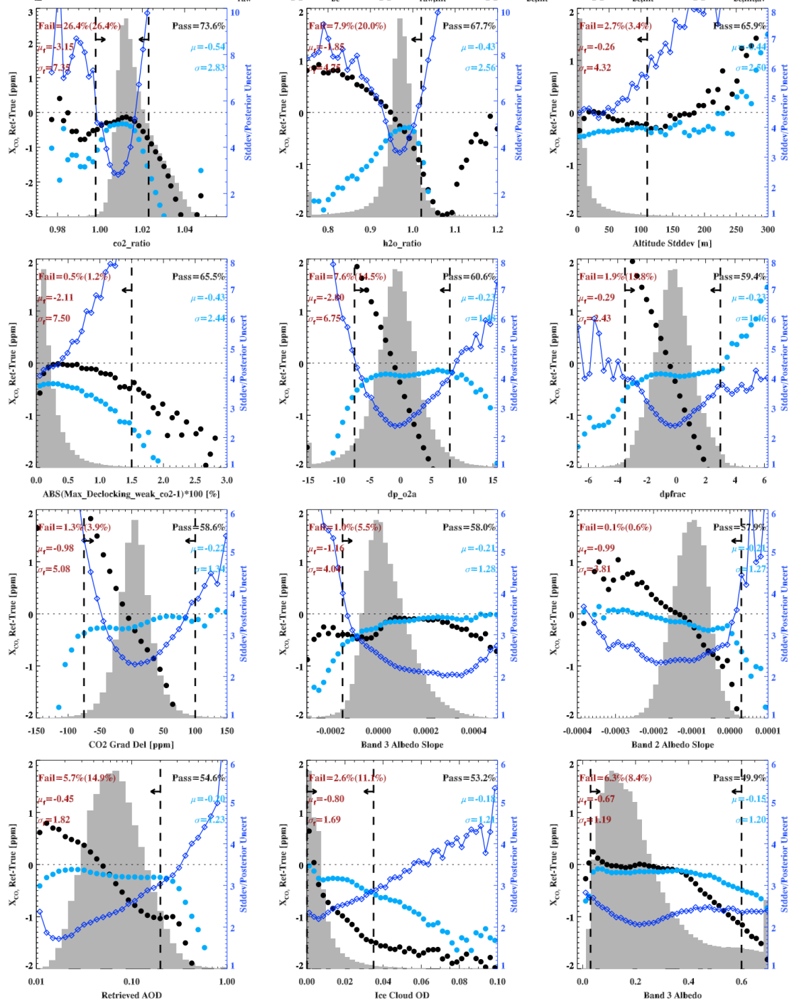
Figure 3-4. Bias & Stddev of error as a function of selected outlier filtering variables for land observations. Here, the error is derived using the model comparison.
