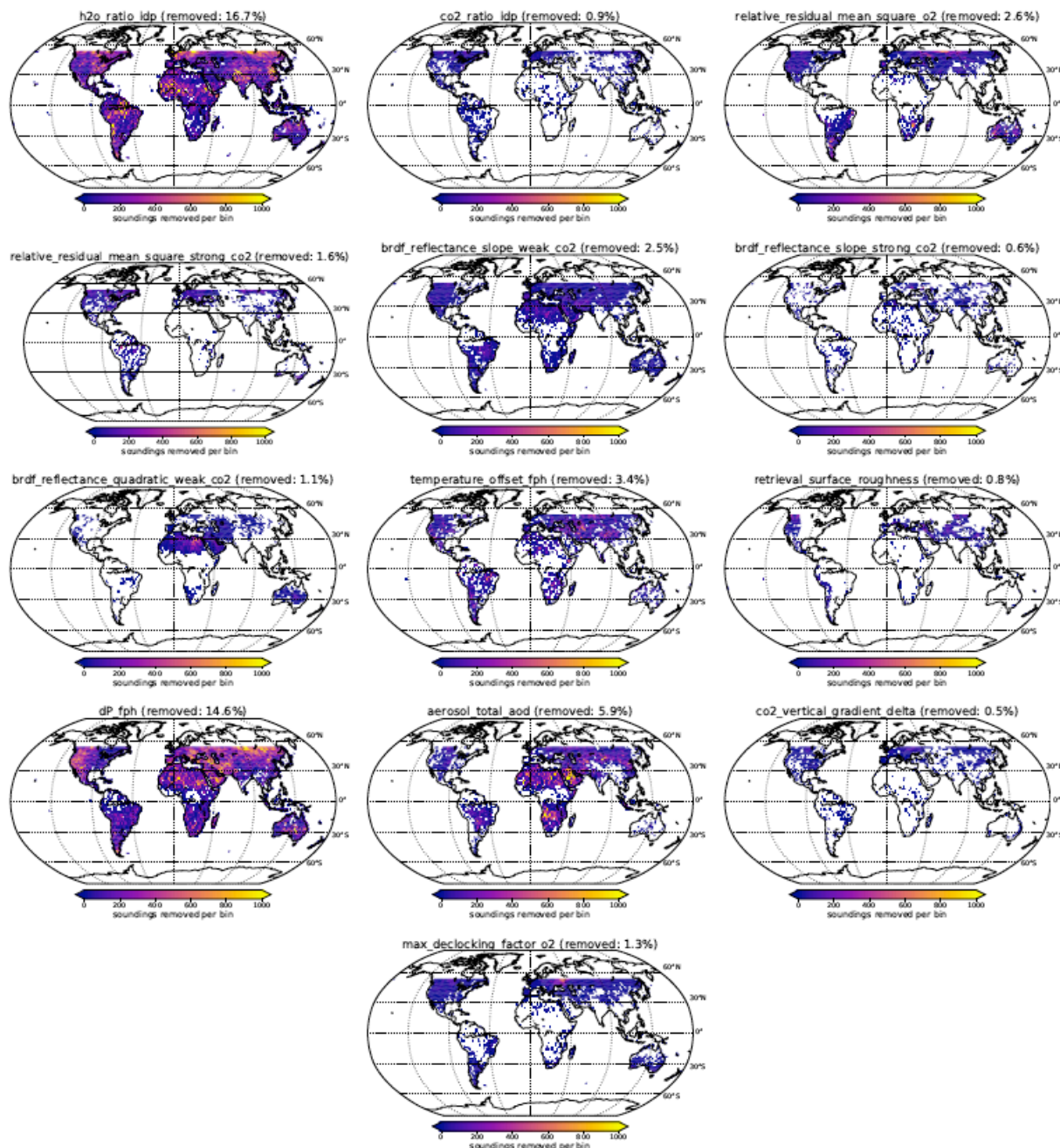
Figure 4-1. Land nadir soundings removed after each filter is applied sequentially. Soundings are aggregated into 2X2 bins.
