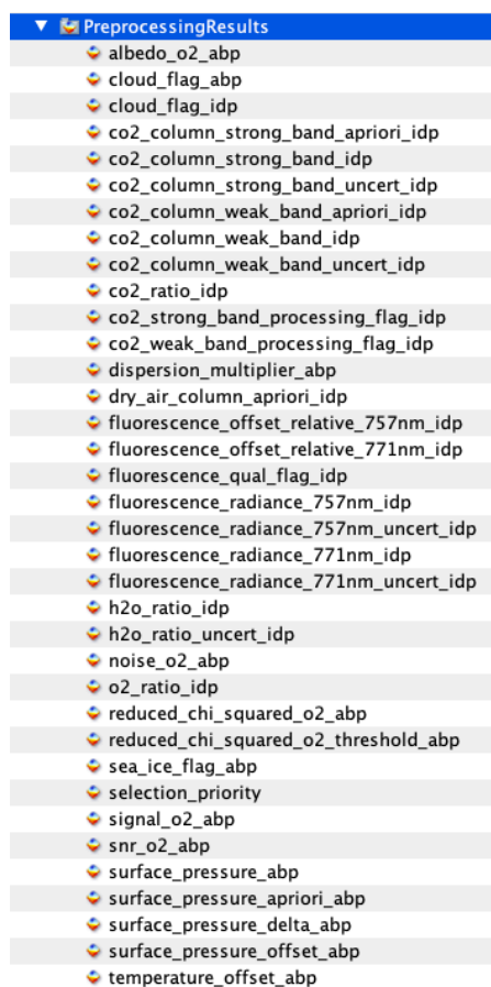
Figure 7-1. Screenshot of an HDFView look at the ABO2 preprocessor file.
