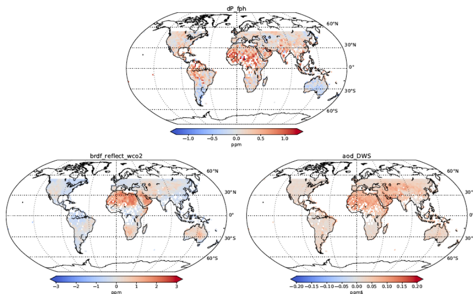
Figure 4-2. Contribution of the dP, albedo_wco2 and aod_DWS bias correction terms to raw X_{CO_2} for soundings over land. Soundings are aggregated into 2^\circ \times 2^\circ bins.
