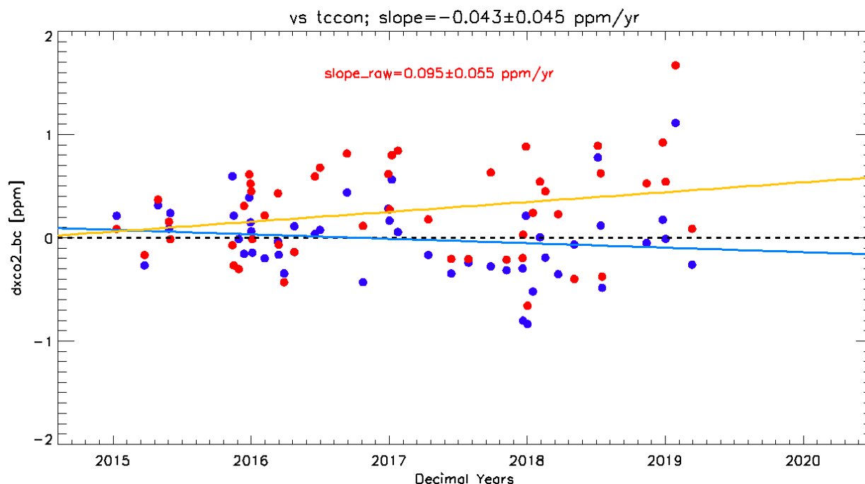
Figure 3-5. Sample linear Fit of OCO-2 V10 minus TCCON vs. time, to determine possible spurious time trend. Bias-corrected XCO 2 differences are shown in (Blue); raw XCO 2 differences are shown in (Red).
