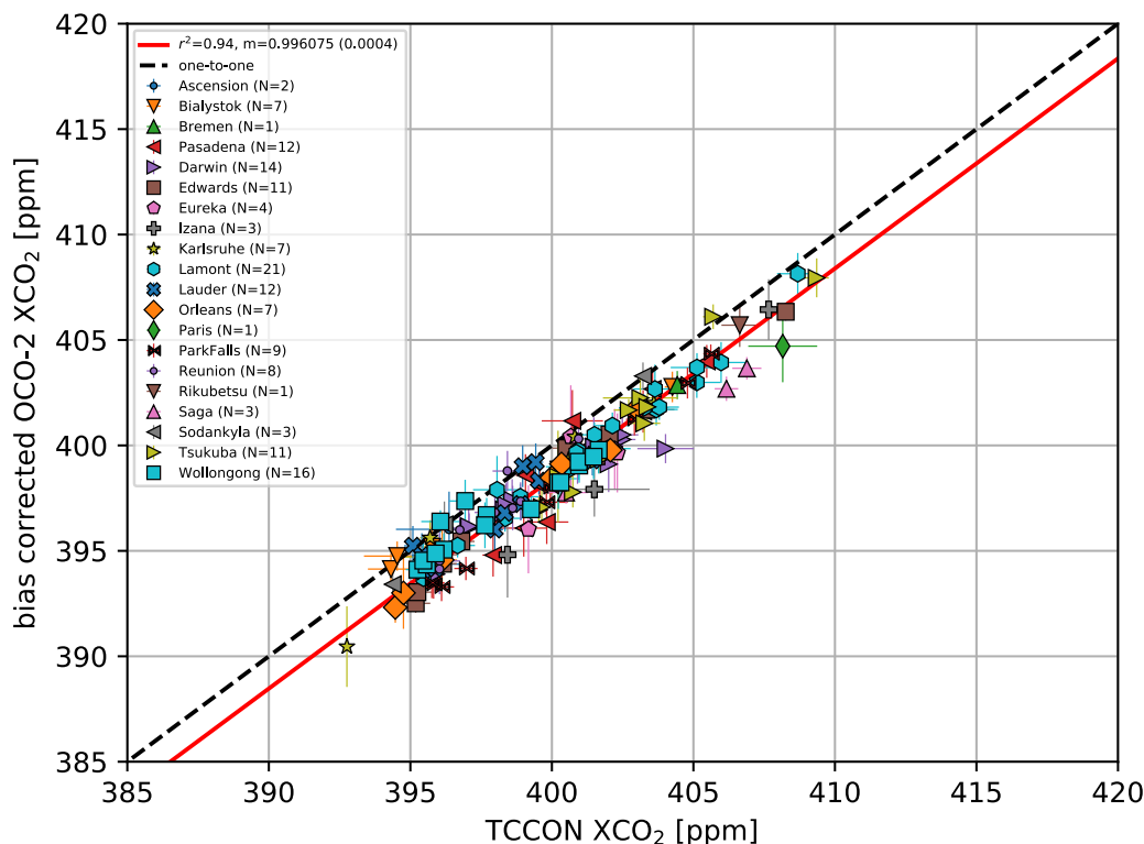
Figure 3-3. Linear Fit of OCO-2 V10 to TCCON X_{CO2} for a subset of target mode overpasses of TCCON sites. Both Quality Filtering as well as the feature and footprint biases have been applied.
