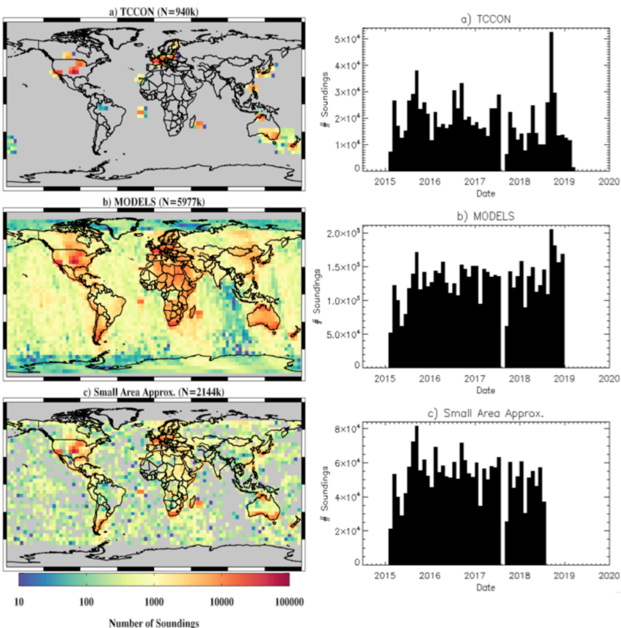
Figure 3-1. Sounding density maps and time series of soundings for the three V10 training data sets.
