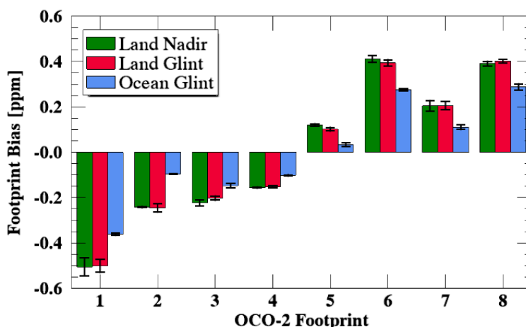
Figure 3-2. Footprint Bias per viewing mode. The land nadir and glint biases were set to be the same in the end, as they were statistically indistinguishable, but the ocean glint footprint biases were statistically different and hence set to their own values.
