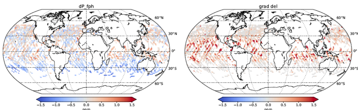
Figure 4-3. Contribution of the dP and co2_grad_del bias correction terms to raw X_{CO_2} for sounding over water. Soundings are aggregated into 2^\circ \times 2^\circ bins.
