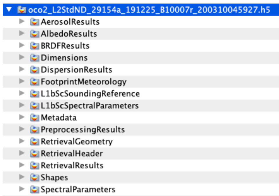
Figure 6-1. Data folders in the L2Std file.
