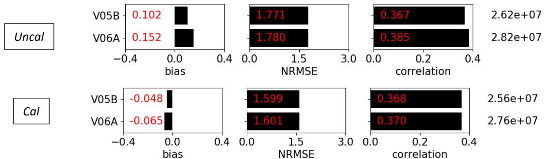
Fig. 3. Bias, normalized root mean square error (NRMSE), and Pearson correlation coefficient for cases where both IMERG and the MRMS-based ground reference meet the 0.2 mm/h threshold) for Uncal (top) and Cal (bottom). The numbers on the right indicate the sample sizes (number of hits). Between V05B and V06A, there is a slight increase in the bias of the uncalibrated estimates, a marginal increase in NRMSE, and a modest increase in the correlation.
