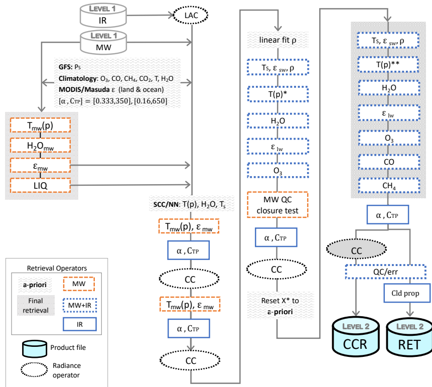
Figure 11. AIRS-team V7 retrieval flow diagram.
