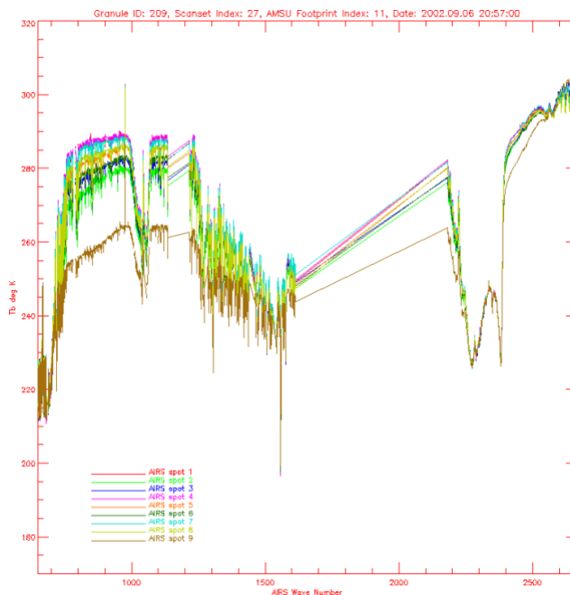
Figure 9. Infrared Radiance Spectra (AIRS) Sept 6, 2002; granule 209; scanline 27; footprint 11
