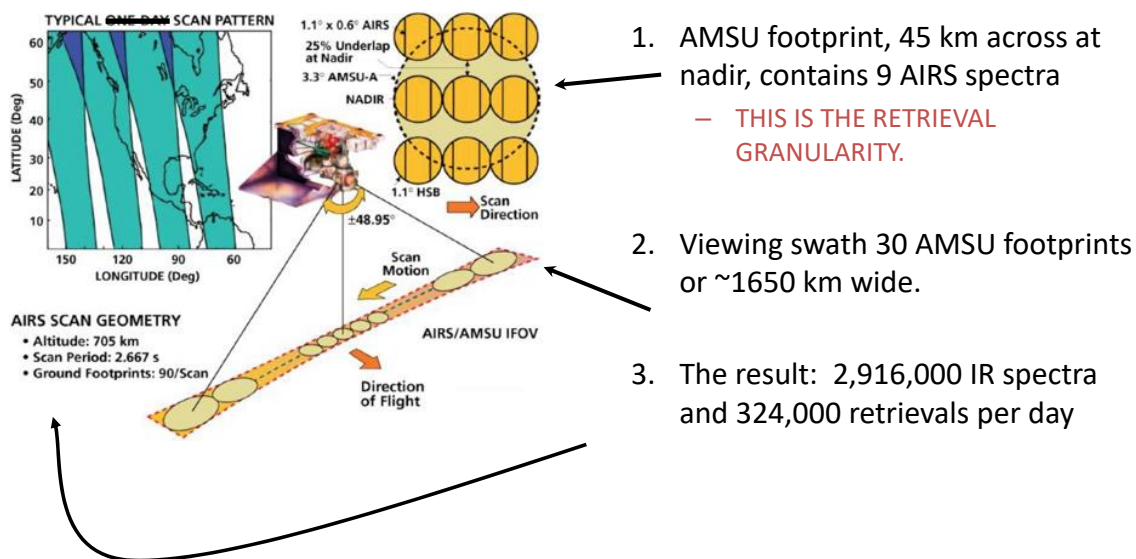
Figure 2. AIRS, AMSU and HSB observations within a single AMSU footprint, and within an orbital swath.
