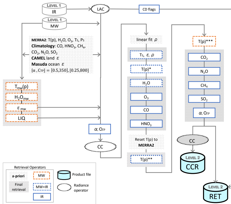
Figure 12. CLIMCAPS retrieval flow diagram. This diagram was originally published in the CLIMCAPS Science Application Guide.
