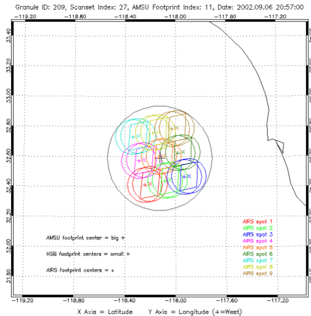
Figure 7: AIRS/AMSU/HSB Footprint Pattern Sept 6, 2002; granule 209; AMSU scanline 27; footprint 11, central (lat,lon) = (32.6°, -118.1°), just west of San Diego, California.
