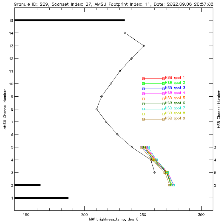
Figure 8. Microwave Radiances (AMSU-A and HSB) Sept 6, 2002; granule 209; scanline 27; footprint 11
