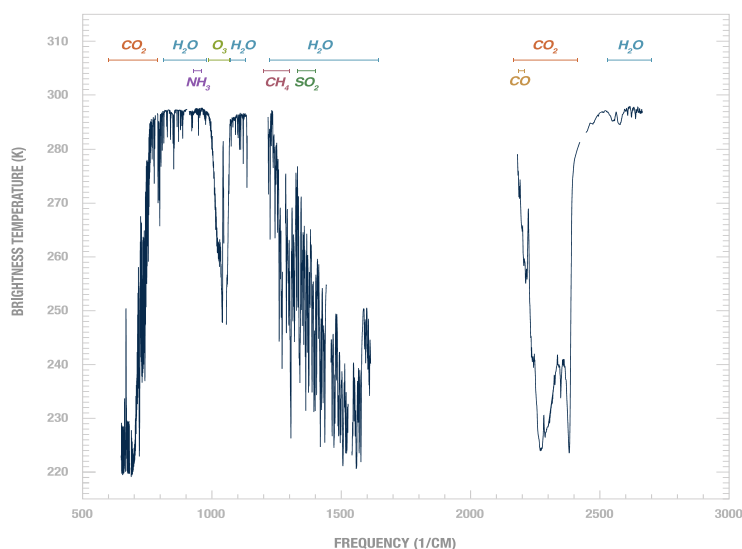
Figure 3. Simulated AIRS spectrum with prominent spectral features marked.
