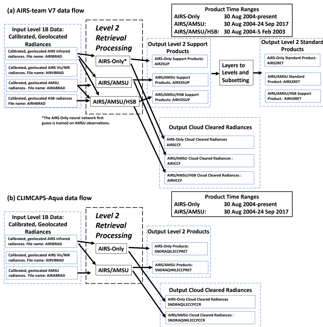
Figure 14. Data flow for the creation of Level 2 products from AIRS Level 1 input data, for the two retrieval systems, (a) AIRS-team V7, and (b) CLIMCAPS-Aqua. Products created by Level 2 retrieval processing are within the rectangular boxes, with blue dashed boxes surrounding similar products from different processing algorithms. Cloud cleared radiances are in separate files from other Level 2 retrieval products. For AIRS-team V7, all quantities in Table 2 are included in the three Level 2 processing types of AIRS-Only, AIRS/AMSU, and AIRS/AMSU/HSB. The product names in Level 2 quantities (AIRS2SUP, etc.) are discussed below in the ‘Short Names’ section. CLIMCAPS-Aqua retrieval products do not include HSB and are not separated into standard and support products.
