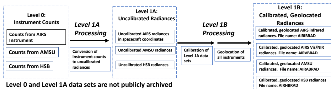
Figure 13. Level 1B processing steps. The product names in Level 1B quantities (AIRSBRAD, etc.) are discussed below.
